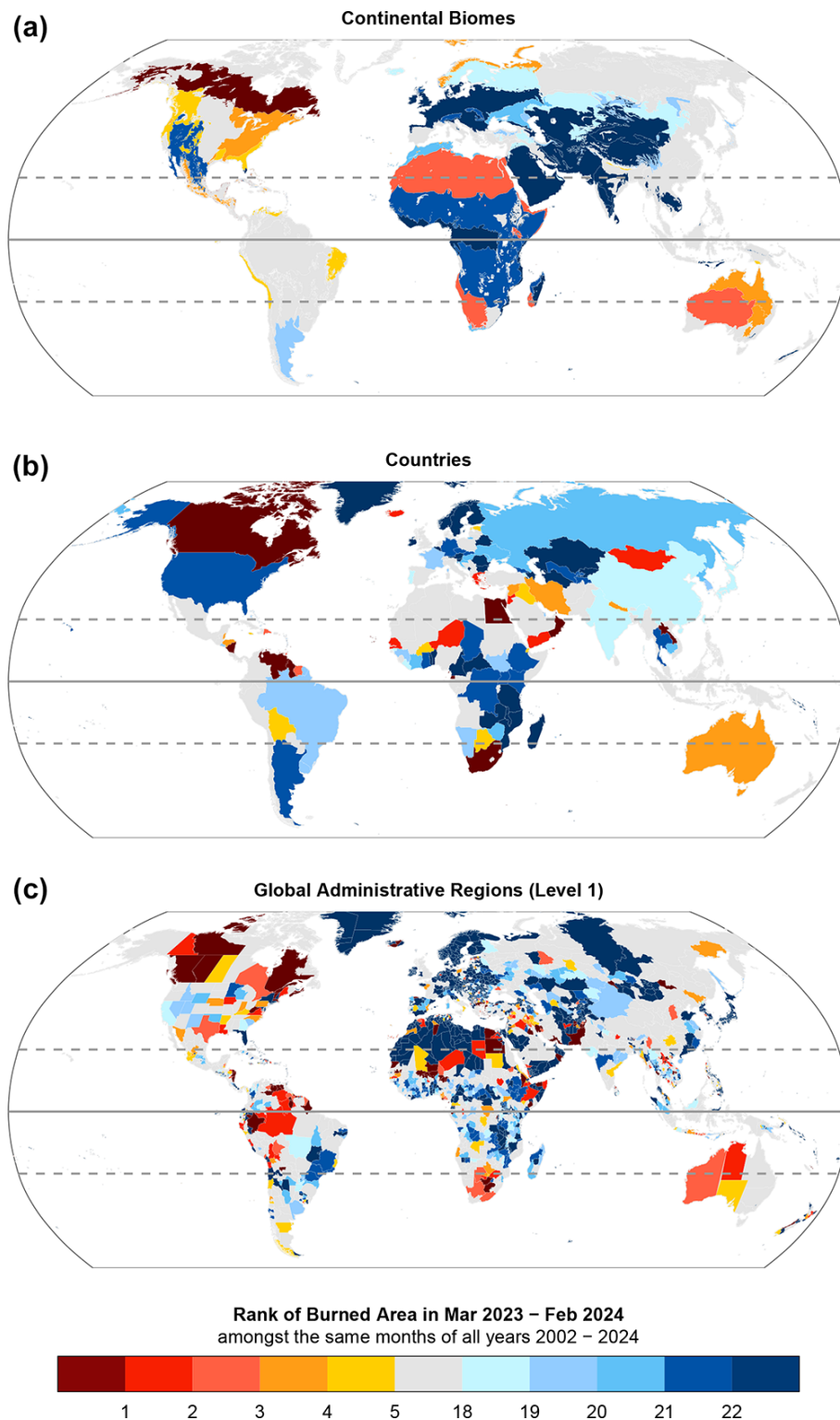
Figure 2. Ranks of BA during March 2023–February 2024 versus previous March–February periods ( n = 23 global fire seasons) for three regional layers: (a) continental biomes, (b) countries, and (c) states or provinces. Results for regions with high-ranking (top 5 years) or low-ranking (bottom 5 years) events are highlighted. The timing of BA anomalies is shown in Fig. S2 in the Supplement.
