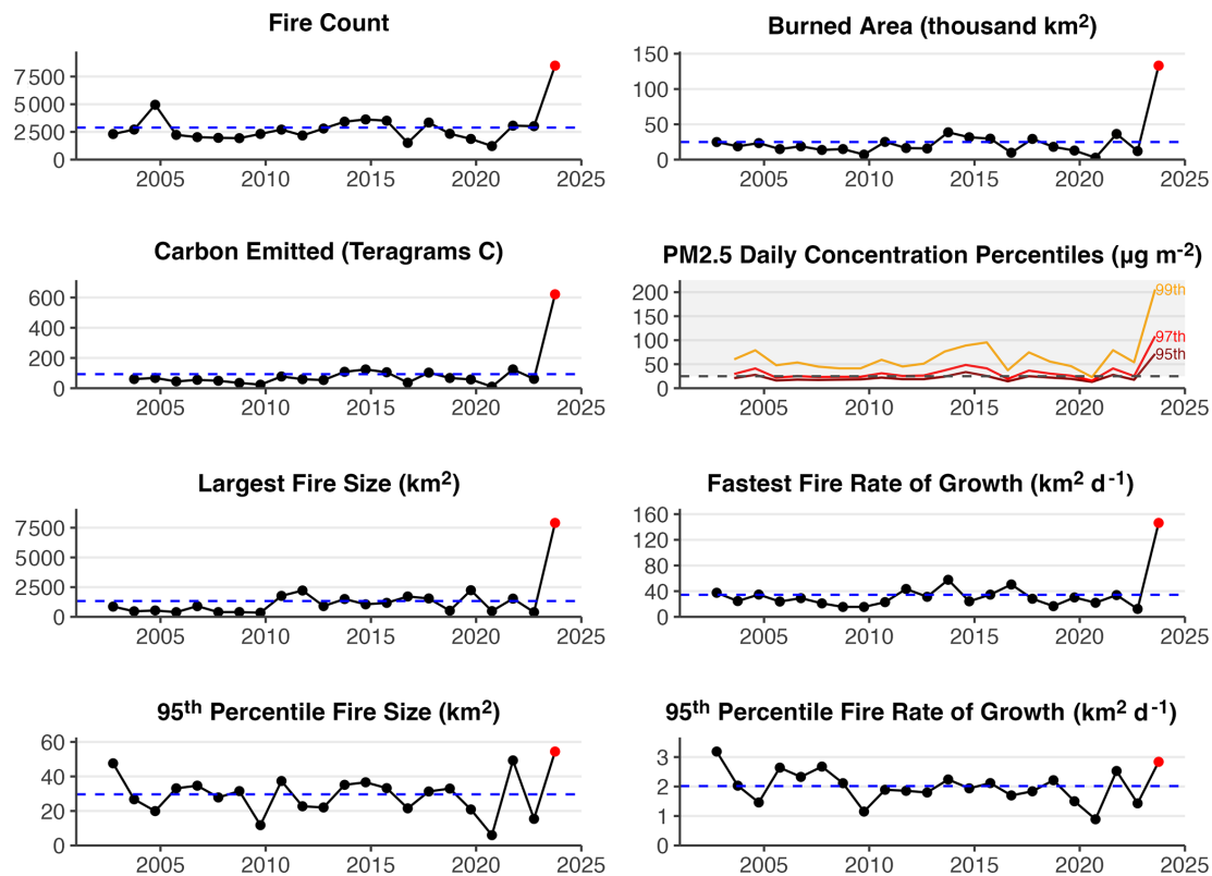
Figure A2. Summary of the 2023–2024 fire season in Canada. Time series of annual fire count, BA, C emissions, \text{PM}_{2.5} daily concentration percentiles (95th, 97th, and 99th), 95th percentile fire size, fastest daily rate of growth, and 95th percentile fire daily rate of growth. Black dots show annual values prior to the latest fire season, red dots the values during the latest fire season, and dashed blue lines the average values across all fire seasons. The \text{PM}_{2.5} daily concentration percentiles are based on area-weighted daily mean surface \text{PM}_{2.5} concentrations within each year across Canada from the CAMS atmospheric reanalysis (Inness et al., 2019). The grey zone marks concentrations exceeding reference levels for 24 h mean \text{PM}_{2.5} concentration in Canada ( 25 \mu\text{g m}^{-3} ; Canadian Environmental Protection Act Federal-Provincial Working Group on Air Quality, 1998).
