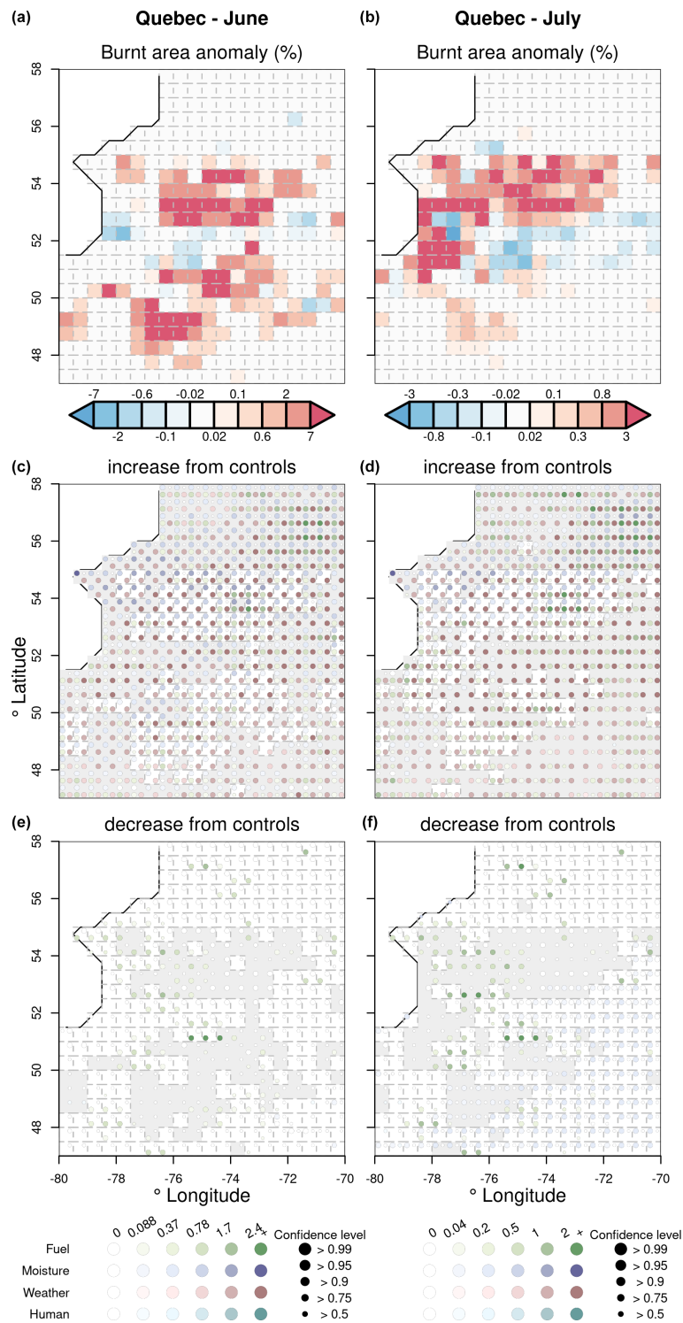
Figure 11. Anomalies in controls during months and regions of high BA in Quebec. The top map of each region shows BA anomalies at 0.5° for that month in 2023 versus the 2014–2023 monthly average. The middle maps look at anomalies in controls that would cause higher BA, with areas not greyed out representing regions with greater than monthly average BA in 2023. The bottom map shows drivers that would have led to lower than normal levels of burning, with areas not greyed out showing lower or non-change from monthly average BA in 2023. Each grid cell has four points: green points show anomalies in fuel load, purple in fuel moisture, red in fire weather, and cyan in humans. This way, we can see if controls acted in unison to cause extreme levels of burning or prevent extreme fires from extending further. The shade of the point shows the most likely expected level of anomaly in that control, while the size shows how confident we are in the direction of the anomaly.
