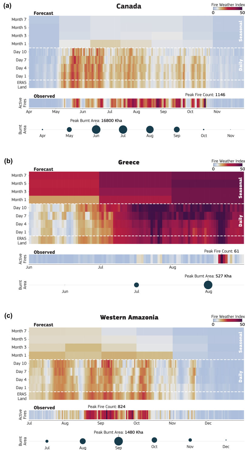
Figure 7. Chicklet plots displaying seamless FWI predictions over time from various forecasting systems of the ECMWF (see Methods). The x axis corresponds to specific dates throughout the year, while the y axis denotes either observations or the time leading up to the date when a forecast was generated. The vertical colour coherence allows for quick identification of the time windows of predictability associated with the observed fire activity provided in terms of both the number of detected active fires in a day and the total predicted area in a month (circles).
