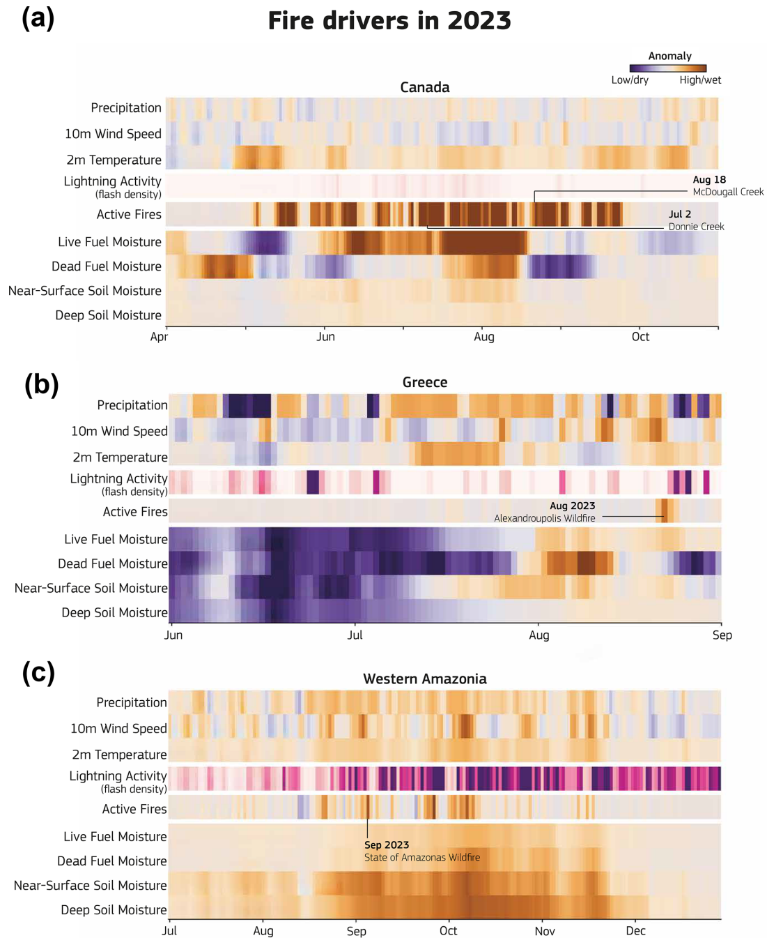
Figure 8. Anomaly driver stripes for the three focal events. The drivers are selected to contextualise the conditions under which the examined events took place. All values are expressed as anomalies compared to the 2003–2021 climatology with the exception of lightning activity, which is expressed as absolute flash density.
